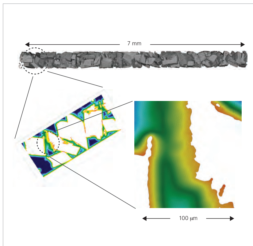
// Reactive transport in a capillary tube packed with crushed calcite from experimental image data. Resolution of the simulation grid (top) is 1 micron, as shown in the second slice of calculated calcite saturation (bottom). (David Trebotich)
