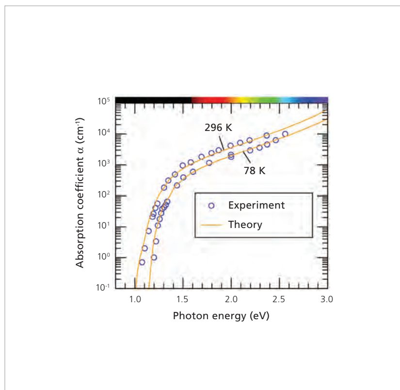
// Absorption spectrum of silicon for two temperatures showing excellent agreement between computed and experimental values. ( J. Noffsinger et al. )
