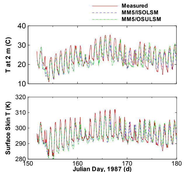
Figure 2. Comparison between FIFE measurements and the MM5/ISOLSM and MM5/OSULSM predictions for June 1987. Shown are the surface skin and 2 m air temperatures.
